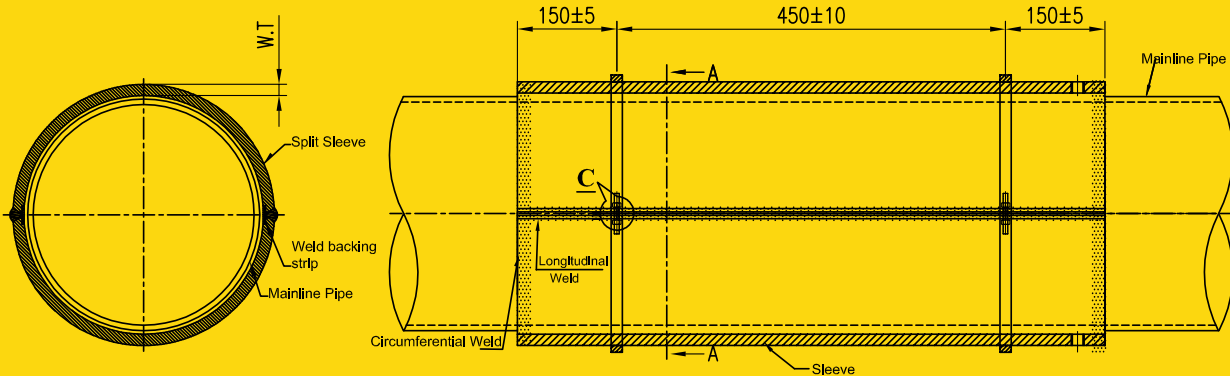
basic drawing reinforcement sleeve
